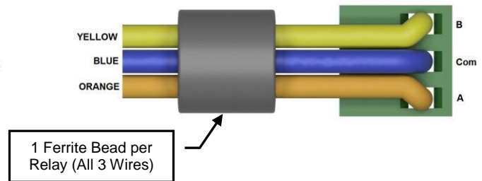
Figure 2 – Relay Wires with Ferrite Beads Installed
