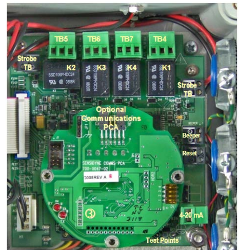
Sensor Interface
