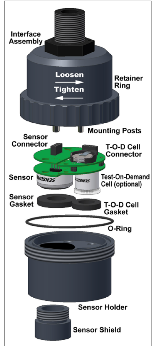
Figure 2-1 Sensor Installation
