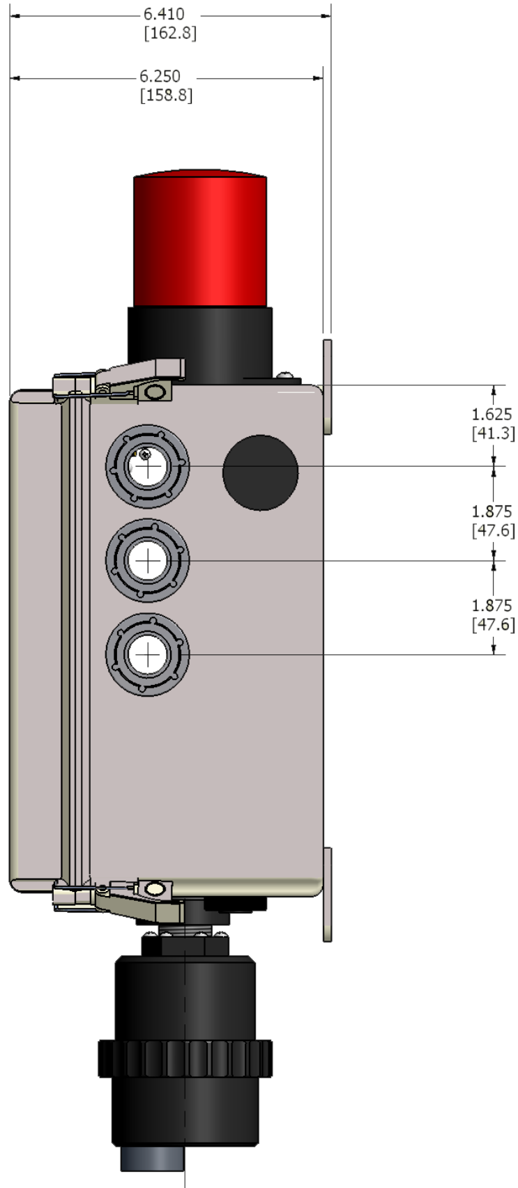
Mounting Dimensions: Monitor With Fiberglass Enclosure
