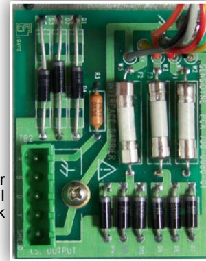
Sensor Terminal Block
