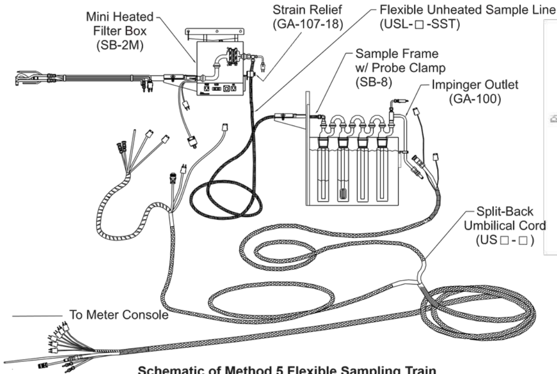
Schematic of Method 5 Flexible Sampling Train
