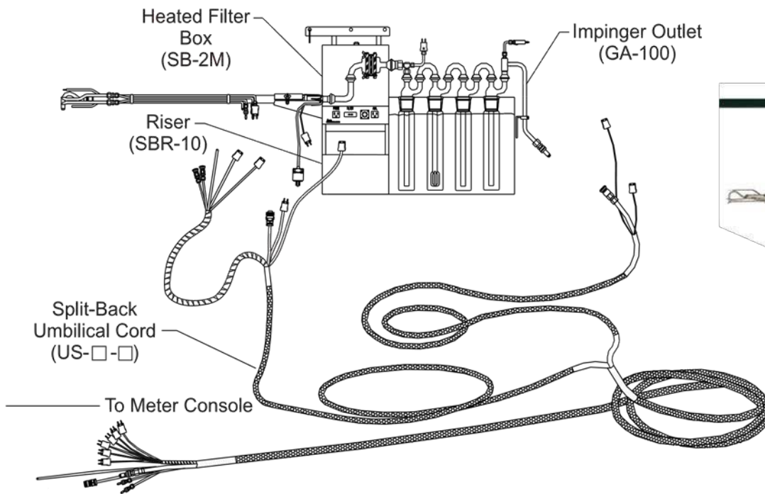
Schematic of Method 5 Rigid Sampling Train
